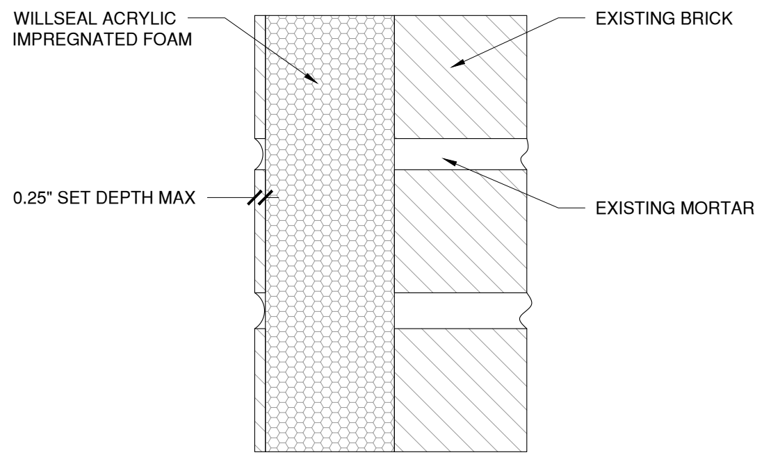
1 SECTION VIEW
